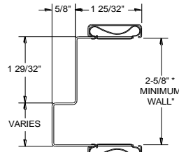
II 1-3/4" FRAME SINGLE RABBET
