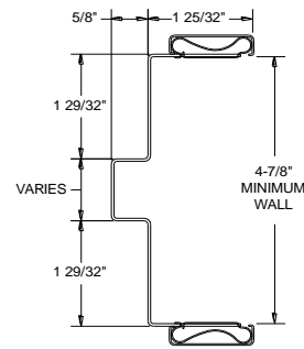
III 1-3/4" x 1-3/4" COMMUNICATING FRAME
