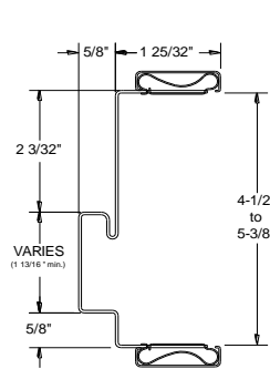
IV 1-3/4" KERF FRAME (KF SERIES)
