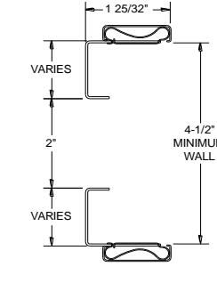
VIII HEADER & POCKET UPRIGHT
