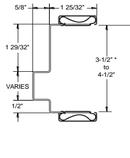
I 1-3/4" FRAME DOUBLE RABBET
