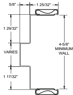
I 1-3/4" FRAME DOUBLE RABBET
