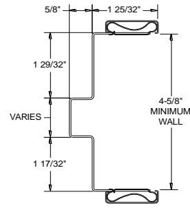
VII 1-3/4" x 1-3/8" COMMUNICATING FRAME
