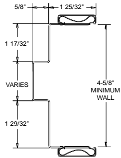
V 1-3/8" FRAME DOUBLE RABBET
