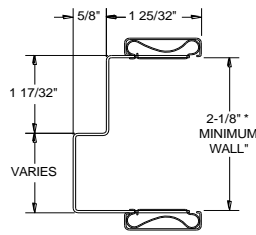
VI 1-3/8" FRAME SINGLE RABBET
