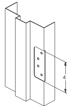
T4R2 4" x 1/4" Radius Template Hinge Backset 3/8" Depth .110"
