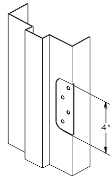
4R5 4" x 5/8" Radius Non-Template Hinge Backset 3/8" Depth .100"
