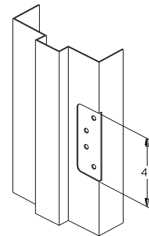
T4R2H 4" x 1/4" Radius Template Hinge Backset 3/8" Depth .125"
