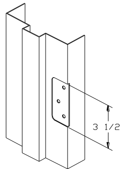
35R2 3 1/2" x 1/4" Radius Template Hinge Backset 9/32" Depth .085"
