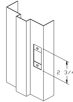
DB Deadbolt Strike Prep Depth .130" # 8-32 Screw
