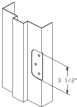
35R5 3 1/2" x 5/8" Radius Template Hinge Backset 9/32" Depth .085"
