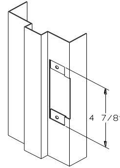
ASA ASA Strike Prep Depth .110" # 12-24 Screw
