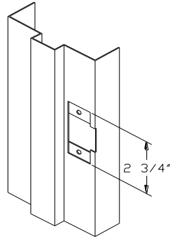
AT Adjustable Strike Prep 1 3/4" Door Depth .130" # 8-32 Screw
