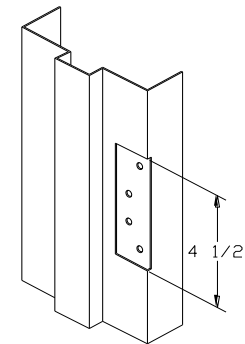
T45 4 1/2" Square Template Hinge Backset 3/8" Depth .134"
