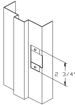
FT Fixed T Strike Prep Depth .110" # 8-32 Screw
