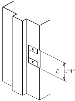
FL 2 1/4" Full Lip Strike Depth .110" # 8-32 Screw
